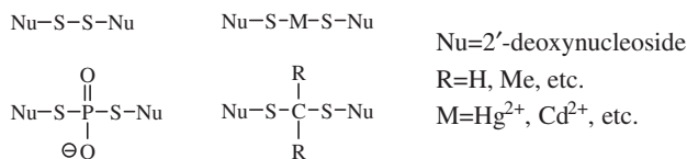
Figure 1. Some Backbones of Novel Nucleic Acids.
