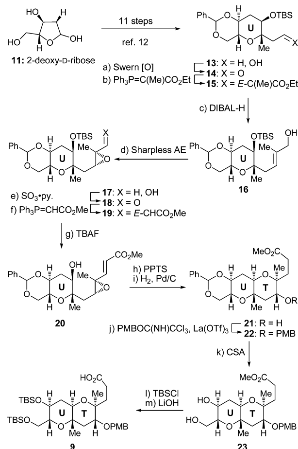
Scheme 1. Synthesis of UT Ring System 9 a
