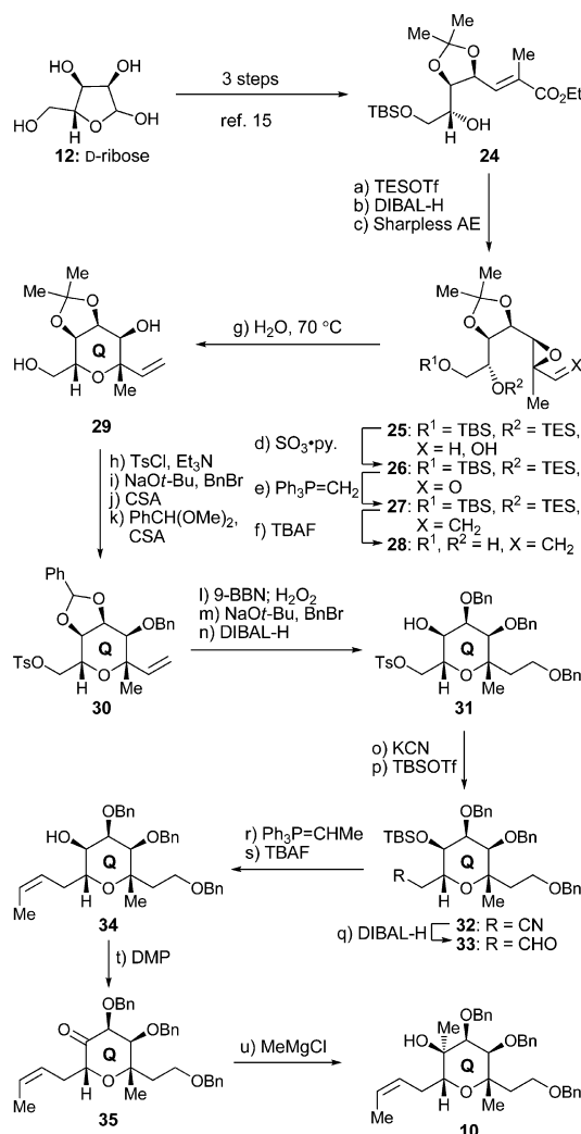
Scheme 2. Synthesis of Q Ring Building Block 10 a
