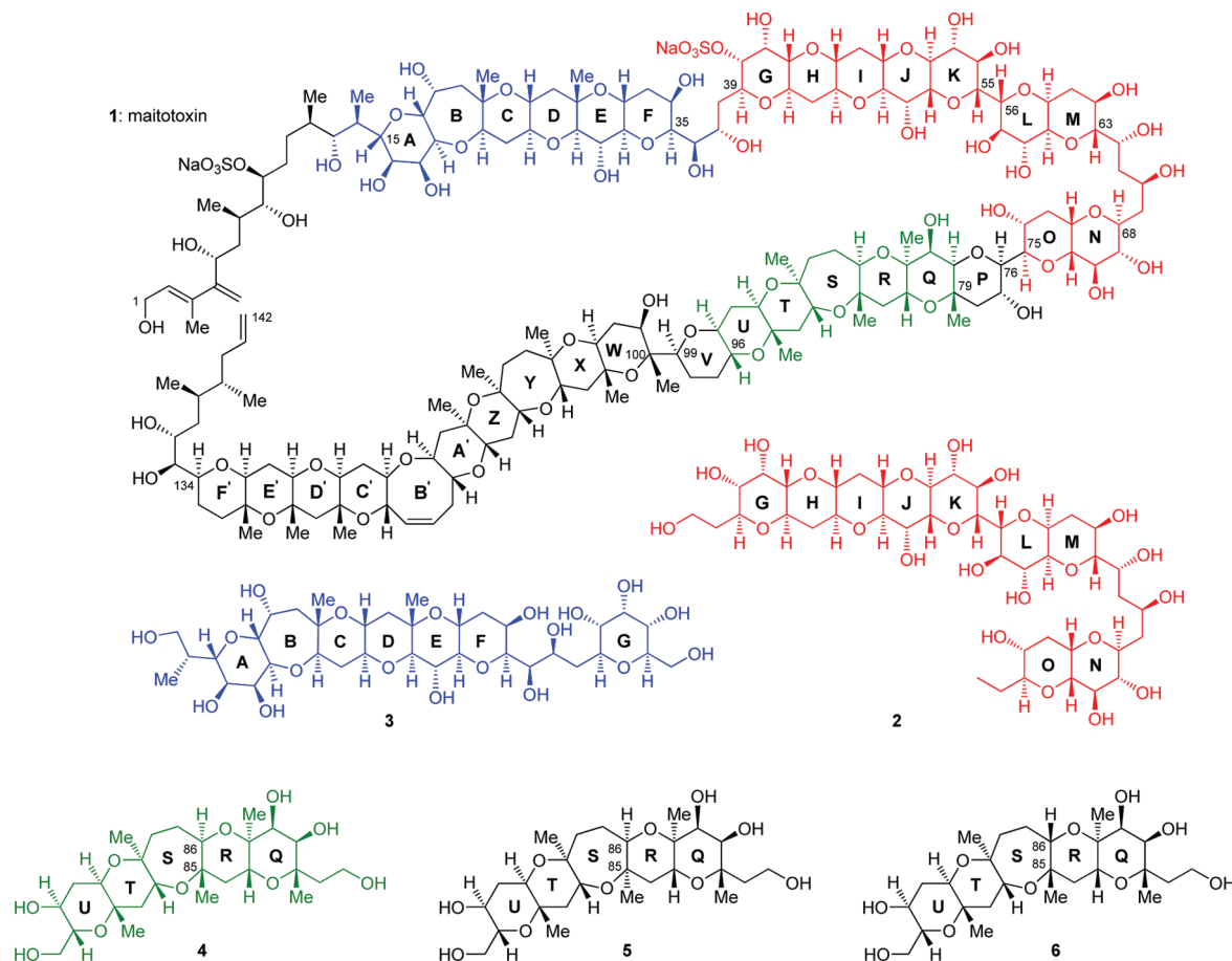
Figure 1. Structures of maitotoxin ( 1 ), previously synthesized maitotoxin domains GHJKLMNO ( 2 ) and ABCDEFGH ( 3 ), targeted QRSTU domain ( 4 ), and its diastereomeric 85- epi -QRSTU domain ( 5 ) and 86- epi -QRSTU domain ( 6 ).
