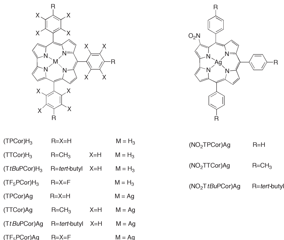
Chart 1. Molecular Structures of the Corroles Studied
