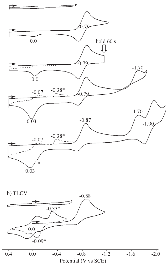
Figure 5. (a) Regular and (b) thin-layer cyclic voltammograms of (TTCor)Ag in pyridine containing 0.1 M TBAP. The electrode reactions involving free \text{Ag}^{\text{I}} and \text{Ag}^0 are indicated by *.
