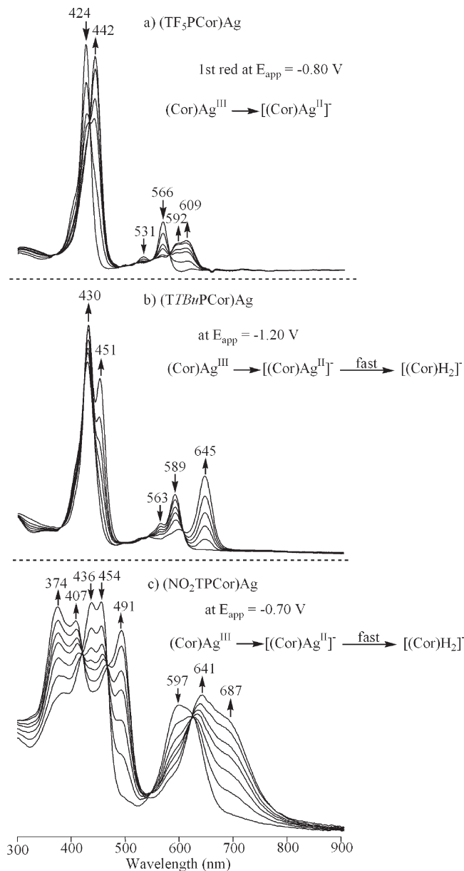
Figure 6. UV-visible spectral changes during the first reduction of (a) ( \text{TF}_5\text{PCor} )Ag, (b) ( \text{tBuPCor} )Ag, and (c) ( \text{NO}_2\text{TPCor} )Ag in pyridine containing 0.1 M TBAP.
