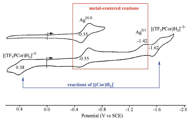
Figure 3. Cyclic voltammograms of (TF 5 PCor)Ag in pyridine containing 0.1 M TBAP.
