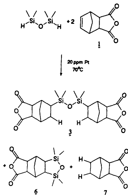
Scheme 1. Synthesis of 3 via tetramethyldisiloxane.
