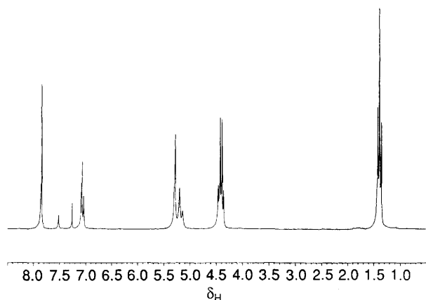
Fig. 1 200 MHz ^1\text{H} NMR spectrum ( \text{CDCl}_3 ) of compound [(\text{EtO}_2\text{C})_8\text{-(py)}_7\text{-O}]_3\text{-[C}_6\text{H}_3(\text{CH}_2)_3\text{]}_2 12
