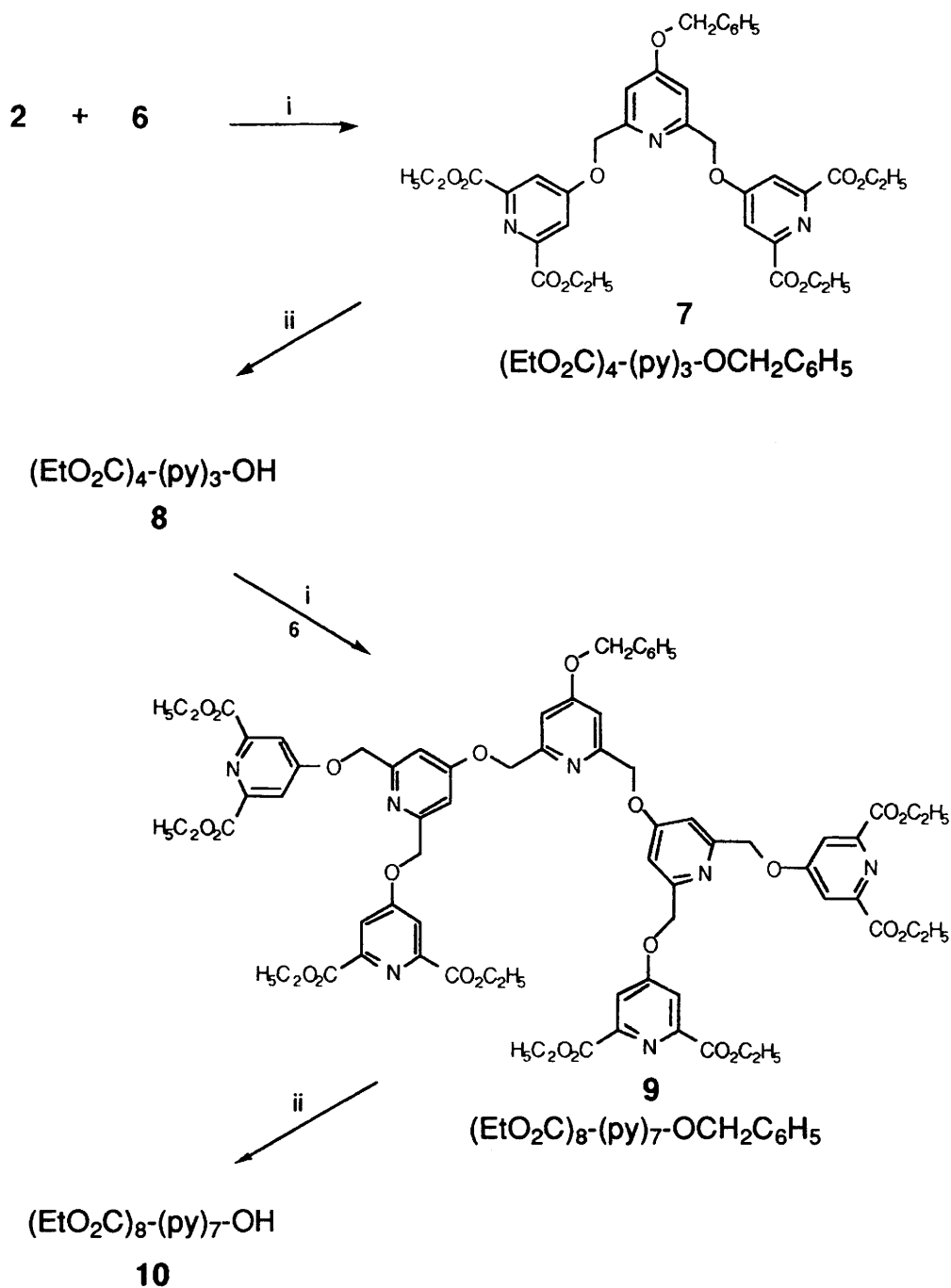
Scheme 2 Reagents: i, K_2CO_3 ; ii, H_2 , Pd/C. Reaction scheme for the synthesis of the ethyl ester-terminated dendritic fragments.
