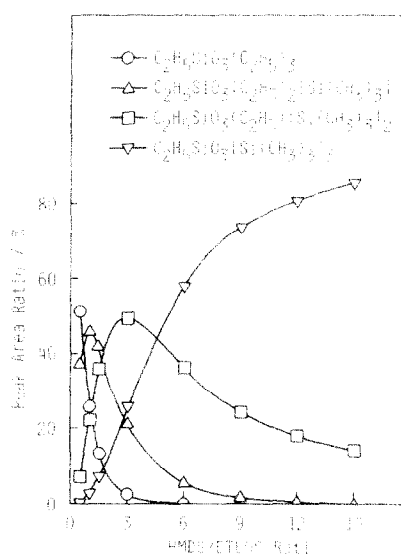
Fig. 3. Effect of HMDS/MTEOS ratio on the peak area ratios of the derivatives from MTEOS( CH_3SiO_3(C_2H_5)_3 ) under Amberlyst 15 treatment at 40°C for 85 h.
