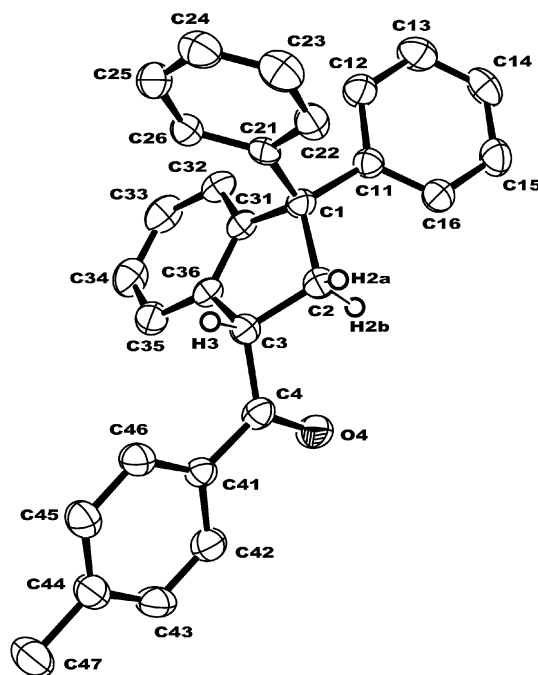
Fig. 4 Molecular structure of 1-(hetero)aryl 3,3-diphenylindane 11e (most hydrogen atoms were omitted for clarity, ORTEP: 50% probability).
