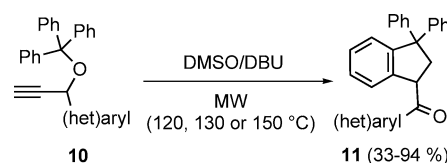
Scheme 4 Microwave-assisted isomerization-Claisen-cyclization domino sequence to 1-(hetero)aryl 3,3-diphenylindanes 11 .
