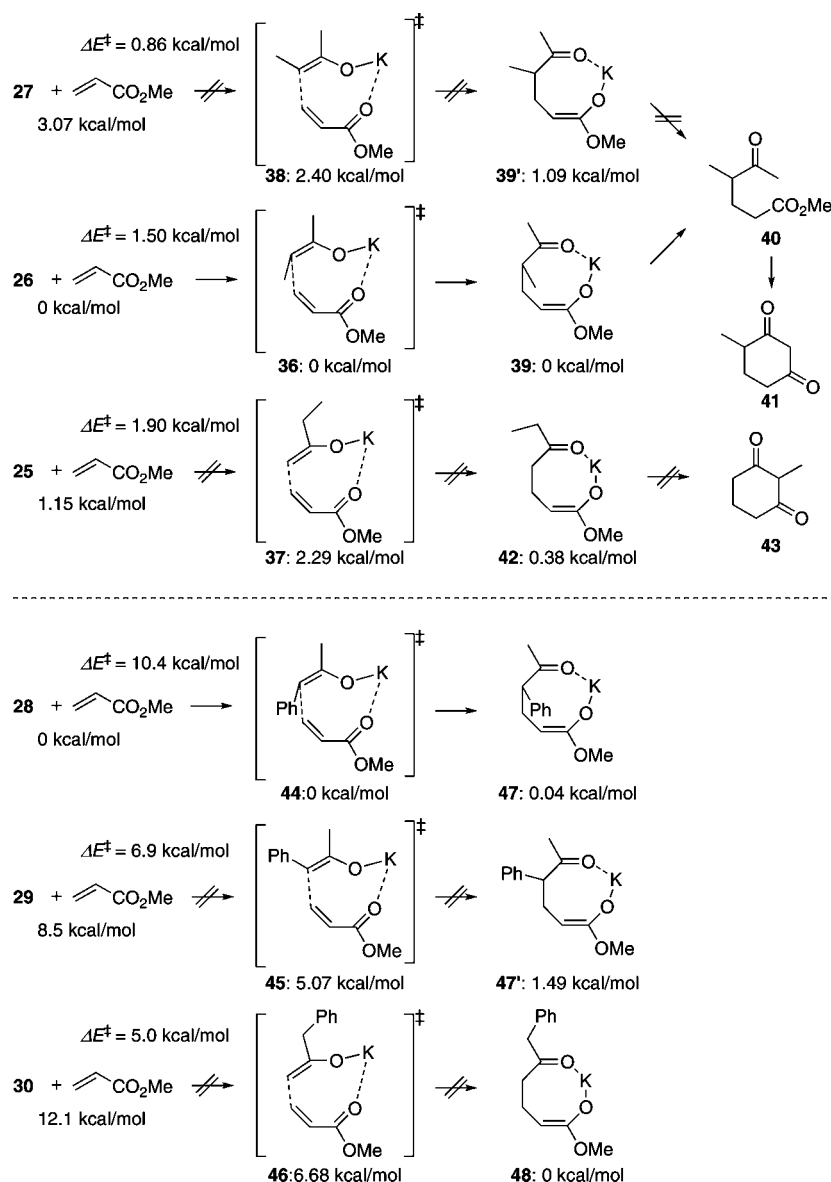
SCHEME 6. Michael Reactions of Enolates 25–30 with Methyl Acrylate (MA) a
