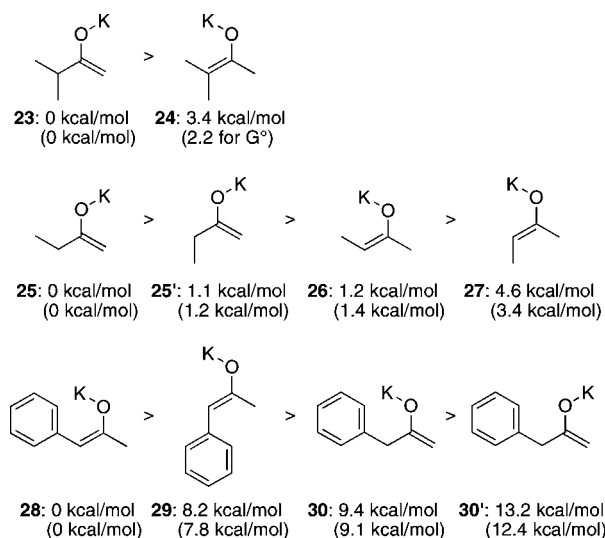
FIGURE 2. Stability orders determined by DFT calculations for some simple enolates 23 – 30 including their conformational isomers ( 25' and 30' ): total electronic energies together with Gibbs free energy indicated in parenthesis.
