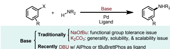
Scheme 1. Mild organic bases for cross coupling reactions in batch and flow.
