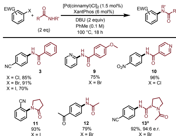
Scheme 4. Selected scope table for the Buchwald-Hartwig amination in the presence of DBU. a
