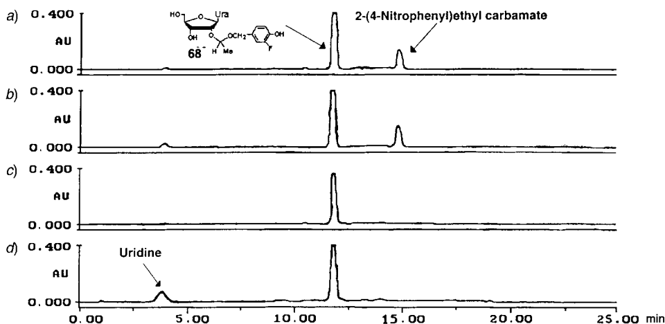
Fig. 1. HPLC Traces of the crude reaction products from 37 after the following treatments: a) 1 \times \text{CHCl}_2\text{COOH}/\text{NH}_3 , b) 10 \times \text{CHCl}_2\text{COOH}/\text{NH}_3 , c) 1 \times \text{CHCl}_2\text{COOH}/\text{DBU}/\text{NH}_3 , and d) 1 \times \text{CHCl}_2\text{COOH}/\text{DBU} , then 9 \times \text{CHCl}_2\text{COOH}/\text{NH}_3 . Column: LiChrospher 100 RP-18, 4 \times 125 mm (Merck); gradient: 0% MeCN (0–2 min) 0–50% MeCN (2–32 min), 50% MeCN (32–40 min) in 0.1M (\text{Et}_3\text{NH})\text{OAc} (pH 7.0); flow rate: 1 ml/min.
