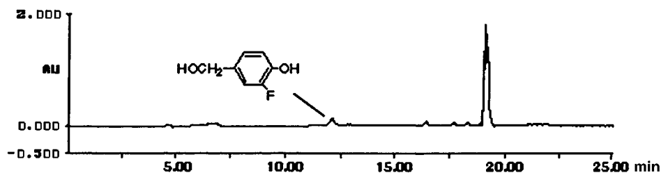
Fig. 3. HPLC Trace of undecameric homouridylylate, after deprotection of [2'-O-[1-[(3-fluoro-4-hydroxybenzyl)-oxy]ethyl]] 10 U 11 by treatment with 3% AcOH for 180 min. Gradient: 0% MeCN (0–2 min), 0–50% MeCN (2–32 min), 50% MeCN (32–37 min), 50% MeCN (37–45 min).
