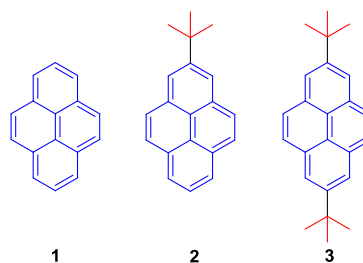
Figure 1. Formulae of compounds 1-3.
