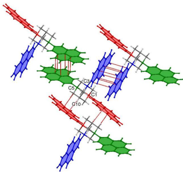
Figure 5. The most important intermolecular interactions formed by 7 in the crystal structure viewed along [100]. Interatomic distances shorter than the sum of the Van der Waals radii presented as red dashed lines.
