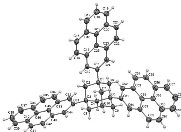
Figure 3. Molecular structure of 7 . Atomic displacement parameters represented at 50% probability level. C atoms numbered 11 – 26 constitute pyrene I, C atoms 31 – 46 constitute pyrene II and C atoms 51 – 66 constitute pyrene III moieties.
