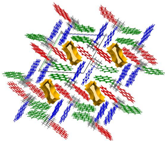
Figure 4. Crystal packing of 7 viewed in [100] direction. Pyrene I, II and III are highlighted in red, blue and green. The disordered molecules of chloroform occupy channels highlighted in yellow.
