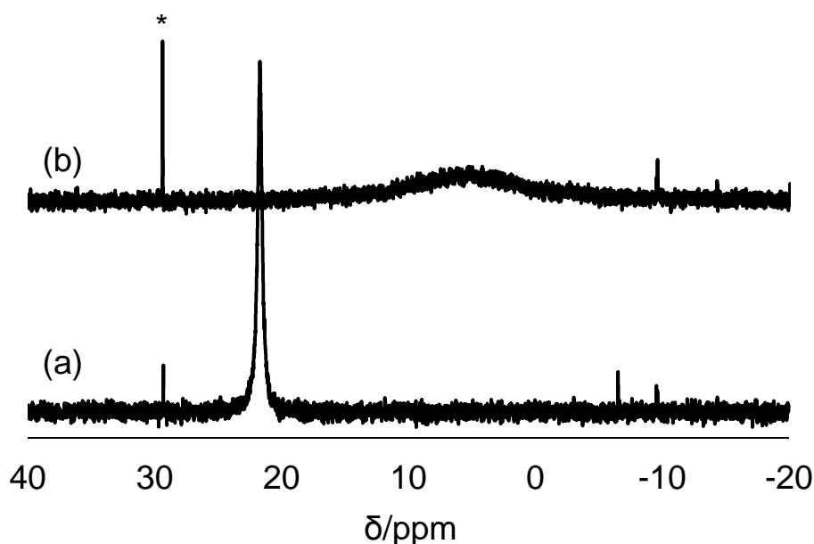
Figure 1. ^{31}\text{P}\{^1\text{H}\} NMR spectra of the [\text{IrCl}(\text{COD})]_2 + \text{PPh}_3 reaction in isopropanol (aliquot evaporated to dryness and residue redissolved in \text{CDCl}_3 ). (a) P/Ir ratio = 1. (b) P/Ir ratio = 2. The starred resonance ( \delta 29.3) is due to a small amount of \text{Ph}_3\text{PO} impurity.
