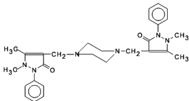
N,N'-bis(antipyrilmethyl)piperazine (BAMP)
