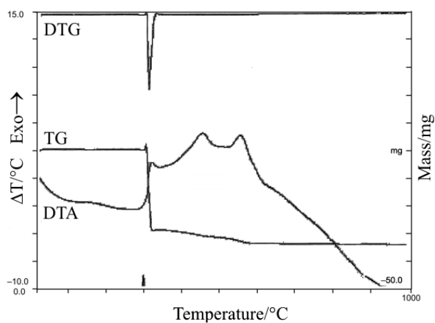
Fig. 2 Thermoanalytical curves of complex 2
