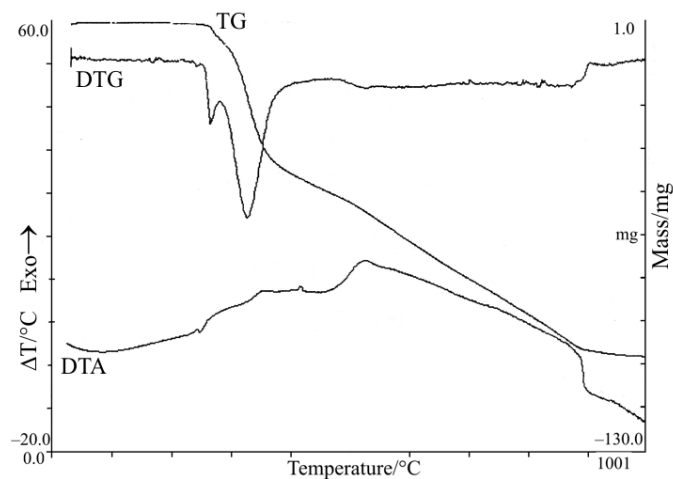
Fig. 5 Thermoanalytical curves of complex 4
