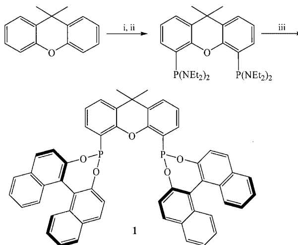
Scheme 1. Synthetic route to compound 1 : i) n BuLi, TMEDA, Et 2 O, −40 °C, 16 h; ii) ClP(NEt 2 ) 2 , pentane, −60 °C, 16 h; iii) 2,2'-dihydroxy-1,1'-binaphthyl (2 equiv.), toluene, tetrazole, Δ T , 1 day
