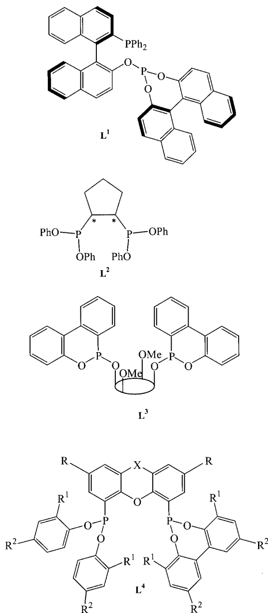
Figure 1. Representation of several reported literature ligand systems: L 1 ) Nozaki's BINAPHOS; L 2 ) cyclopentane-based diphosphonites by Dahlenburg; L 3 ) calix[4]arene-derived diphosphonite of Schmutzler and Börner (the ellipsoid represents a p - tert -butylcalix[4]arene unit); L 4 ) our own sterically constrained achiral diphosphonites
