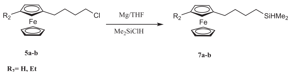
Scheme 3. Synthesis of (4-ferrocenylbutyl)dimethylsilane derivatives.
