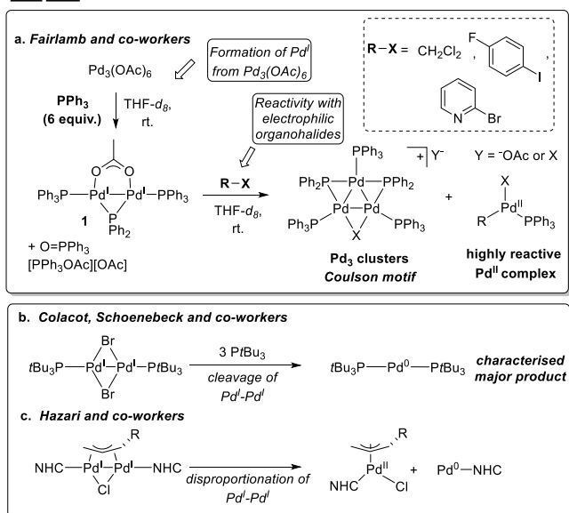
Figure 1. (a) Formation of [\text{Pd}^{\text{I}}_2(\mu\text{-PPh}_2)(\mu_2\text{-OAc})(\text{PPh}_3)_2] complex 1 and reactivity with organohalides. (b, c) Examples of reactivity of \text{Pd}^{\text{I}}\text{-Pd}^{\text{I}} dinuclear complexes.
