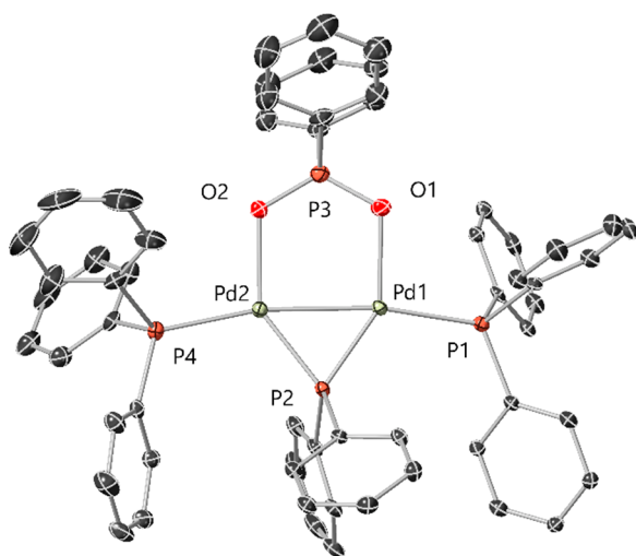
Figure 6. Structure of [\text{Pd}_2(\mu\text{-PPh}_2)\{\kappa_2\text{-O}_2\text{-O-}\mu\text{-P}(\text{O})_2\text{Ph}_2\}(\kappa\text{-PPh}_3)_2] ( 3 ) obtained via a X-ray diffraction of a single crystal grown from THF- d_8 reaction solution of 1 with 2 equiv of \text{PPh}_3 . Selected interatomic distances /Å Pd1–Pd2 = 2.6140(5), P1–Pd1 = 2.2901(12), Pd2–P4 = 2.3095(12), P2–Pd1 = 2.1810(12), P2–Pd2 = 2.1888(12), Pd1–O1 = 2.162(4), Pd2–O2 = 2.186(4), O1–P3 = 1.507(4), O2–P3 = 1.529(4). Selected interatomic angles /° O1–P3–O2 = 120.7(2), Pd1–P2–Pd2 = 73.48(4). H-atoms not shown.
