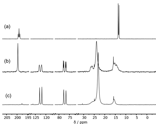
Figure 2. ^{31}\text{P}\{^1\text{H}\} NMR ( \text{THF-}d_8 , 25 ^\circ\text{C} , 203 MHz) showing reaction of [\text{Pd}^{\text{I}}_2(\mu\text{-PPh}_2)(\mu_2\text{-OAc})(\text{PPh}_3)_2] 1 with n\text{PPh}_3 . (a) Authentic 1 ; (b) [\text{Pd}^{\text{I}}_2(\mu\text{-PPh}_2)(\mu_2\text{-OAc})(\text{PPh}_3)_2] 1 + 1 equiv of \text{PPh}_3 after 0.5 h; (c) [\text{Pd}^{\text{I}}_2(\mu\text{-PPh}_2)(\mu_2\text{-OAc})(\text{PPh}_3)_2] 1 + 2 equiv of \text{PPh}_3 after 0.5 h. Note: the spectral window has been shortened, as shown by the double diagonal lines on the chemical shift scale line.
