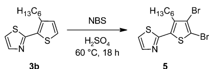
Scheme 3. Bromination of Compound 3b with NBS in Concentrated \text{H}_2\text{SO}_4
