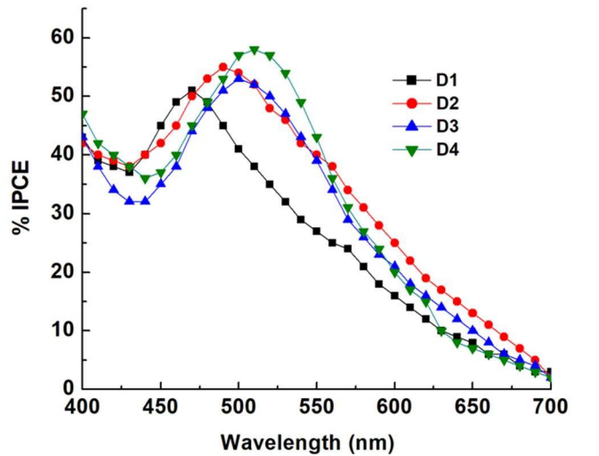
Fig. 9 IPCE plots for the dyes D1 to D4.
