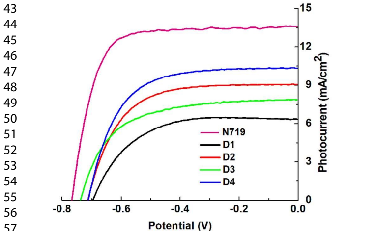
Fig. 8 J–V curves for DSSCs based on dyes D1 to D4 sensitized photoelectrodes
