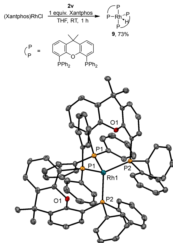
Figure 2. Synthesis and Solid-State Structure of (Xantphos) 2 Rh(H) ( 9 )
