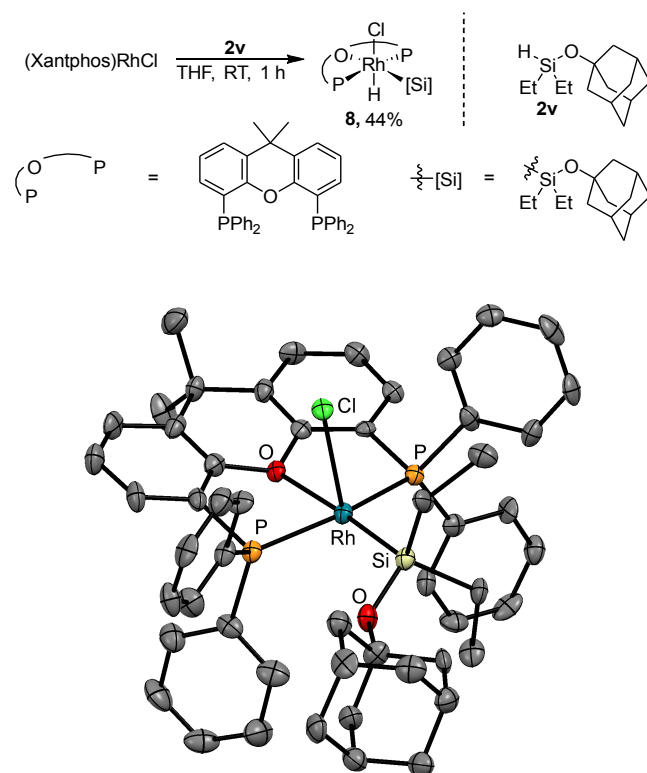
Figure 1. Synthesis and Solid-State Structure of (Xantphos)Rh(H)(Cl)(SiEt 2 OAd) ( 8 )
