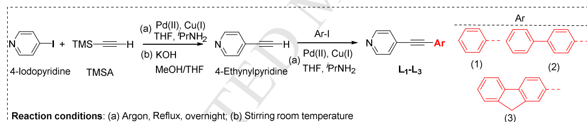
Scheme 1: Synthesis of 4-arylethynylpyridine ligands ( L 1 -L 3 ).
