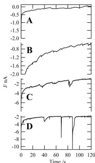
Figure 3: Chronoamperograms (CAs) using Cell 1 (5mM Fc) with 5nm diameter Pt-NPs dissolved at 1.6 (A and B), 7.0 (C), and 16.0 \times 10^{11} NP L -1 (D) in the aqueous phase. A was recorded after a cyclic voltammogram was made to establish the polarizable potential window, but before any further positive polarization. Curves B-D were recorded after CAs were performed at positive potentials. CA potential steps were from -0.20 to -0.30V.
