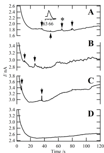
Figure 2: Chronoamperograms (CA) using Cell 1 (5mM Fc) with a potential step from -0.20 to 0.20V with 5, 30, and 50nm diameter Pt-NP (1.6×10 11 NP L -1 ) for curves A-C, respectively (D: no NP added); inset is a typical current spike as marked with an *. Arrows: presumed current spikes.
