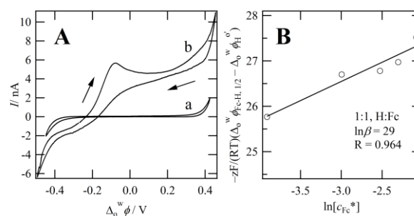
Figure 1. (A) Cyclic voltammograms in Cell 1 without (curve a) and with (curve b) 50mM ferrocene (Fc) with no NP added. (B) Trend of -zF/(RT)(\Delta_o^w \phi_{Fc-H^+, 1/2} - \Delta_o^w \phi_H^+) versus \ln[c_{Fc}^*] .
