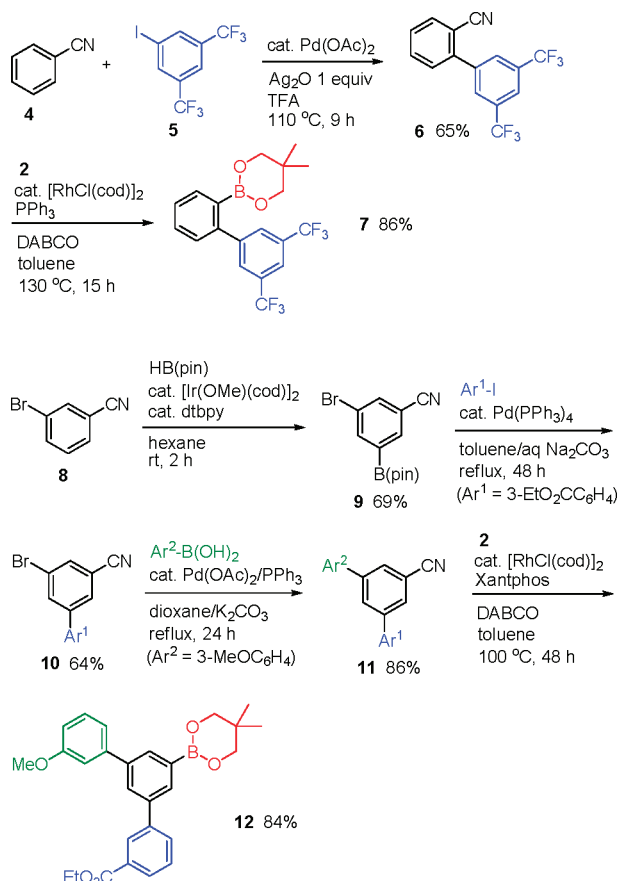
Scheme 3. Synthetic Applications
