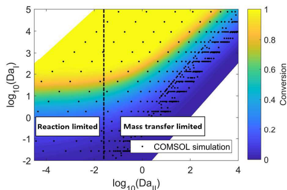
Fig. 4. COMSOL simulation of hydrogenation of nitrobenzene with ethanol as solvent in the membrane reactor. The residence time, carbon cloth thickness, and reaction kinetic constant are varied to obtain different values of Da_I and Da_{II} . Hydrogenation pressure: 2.8 MPa. Carbon cloth layer dimension: length (30 mm) \times width (12 mm) \times thickness (0.05 mm – 3 mm). Membrane thickness: 40 \mu m. The reaction kinetics are available from reported literature, and changing the kinetic constant corresponds to the change of catalyst loading or reaction temperature. 32
