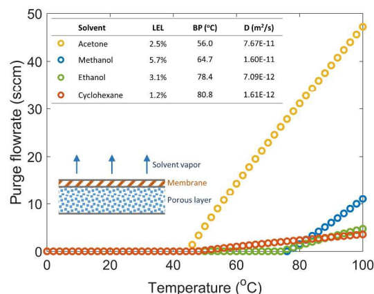
Fig. 2. Required purge stream flowrates for various reaction temperature and solvents. The inserted tables shows the LELs in pure oxygen, boiling points (BP), and diffusion coefficients at 25 °C of the studied solvents.
