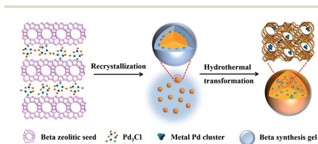
Scheme 1 Illustrations of preparation procedures for Pd 3 @Beta through premade Pd 3 Cl clusters.
