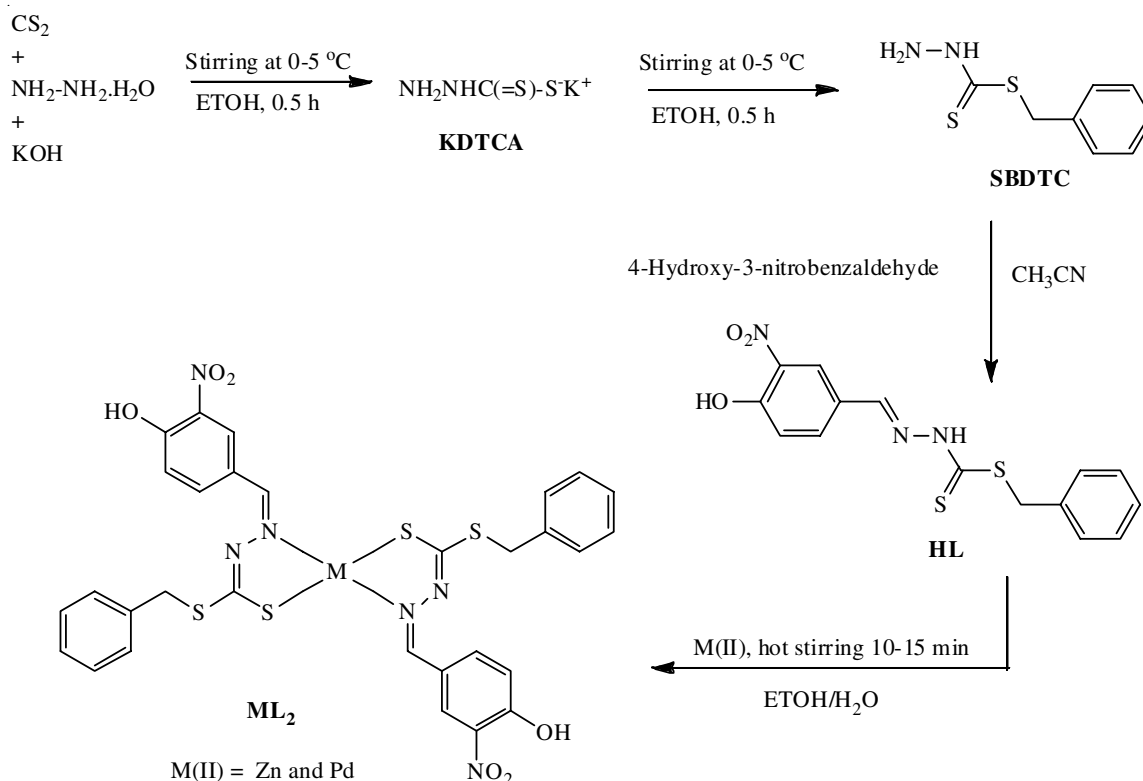
Scheme-I: Synthesis of Schiff base (1) and its metal complexes (2-3)
