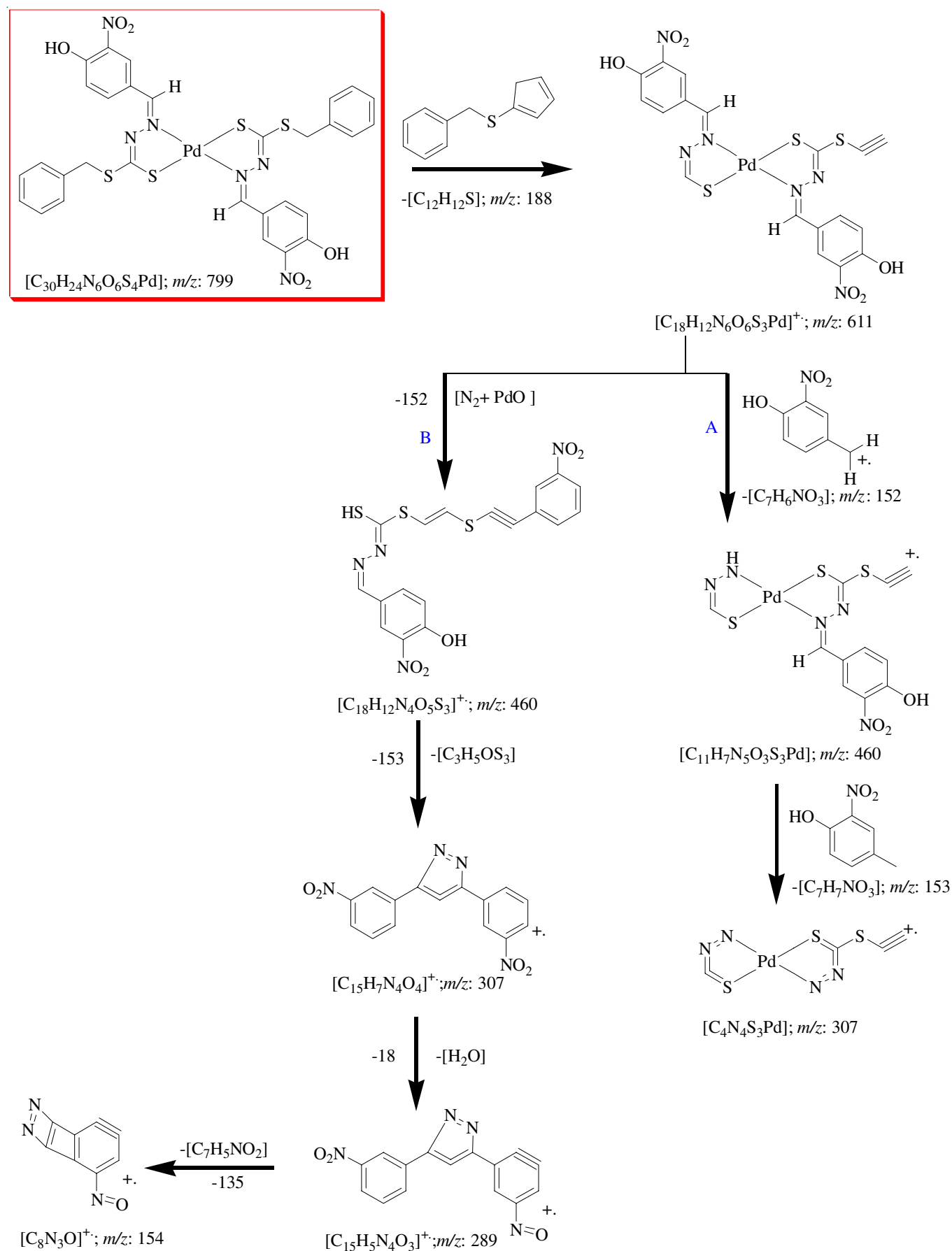
Scheme-IV: Mechanism of fragmentation of Pd(II) complex (3) by low resolution mass spectroscopy
