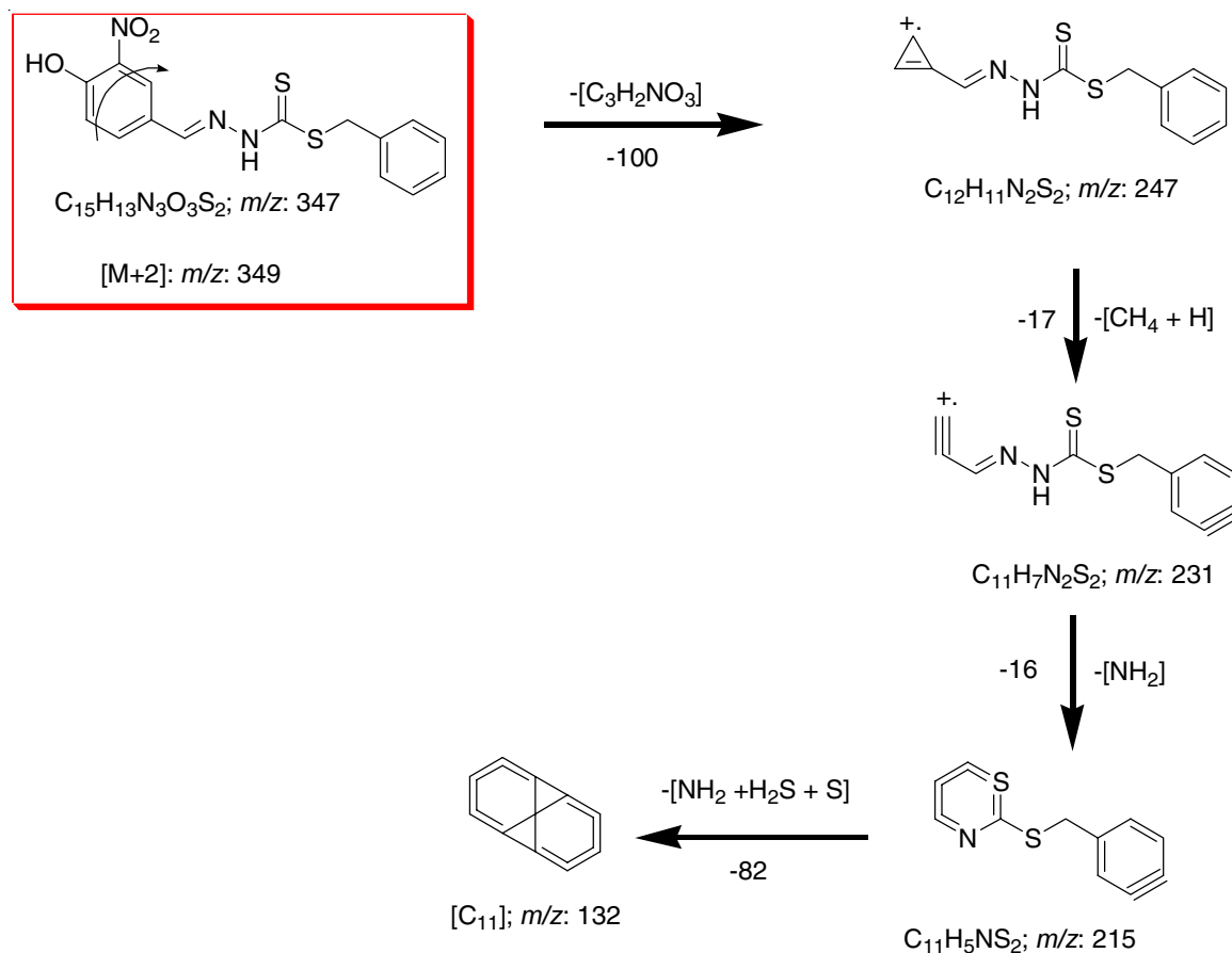
Scheme-II: Mechanism of fragmentation of Schiff base (1) by mass spectroscopy
