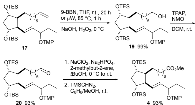
Scheme 6 Transformation of olefin 17 to orthogonally protected ester 4 .
