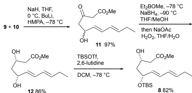
Scheme 3 Preparation of cyclization precursor 8 .
