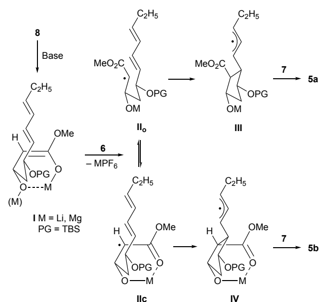
Scheme 4 Course of the radical cyclization/oxygenation of ester 8 .
