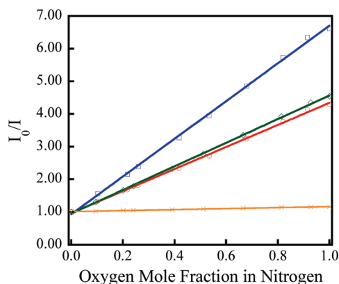
Figure 3. Stern–Volmer plots ( I_0/I ) vs mole fraction of oxygen in nitrogen) for typical samples of 1 (green diamonds), 2b (blue squares), 3b (red circles), and 3c (orange x); the lines are the appropriate linear regression fits ( R^2 = 0.9994, 0.9995, 0.9993 , and 0.9996 , respectively). Three cycles were collected over a 15 h period for each sample; one cycle is displayed for clarity.
