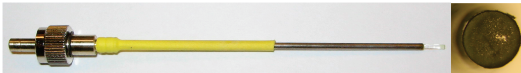
Figure 1. (Left) Fiber optic probe (actual size) used for dissolved O_2 sensing. (Right) Tip of fiber optic with compound at 50\times magnification.
