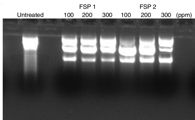
Fig. 1. DNA photo-cleavage activity (FSP = ferrocenyl substituted pyrazoles)
