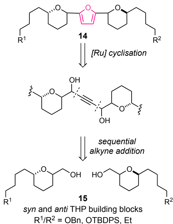
Scheme 1. Bis-tetrahydropyran 2,5-furan retrosynthesis.
