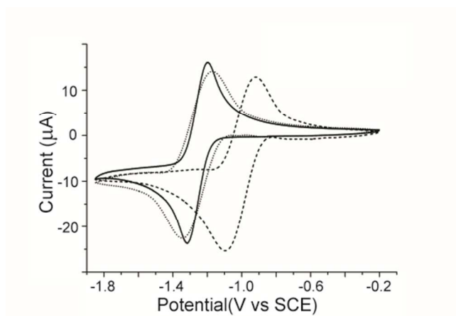
Figure 5. Cyclic voltammograms of 1 in the presence and absence of hydrogen. The solid line shows the voltammogram before exposure of the solution to hydrogen. The dash line shows the voltammograms in a solution saturated with 1 atm hydrogen prepared by sparging immediately preceding measurement. The dotted line shows the voltammogram
