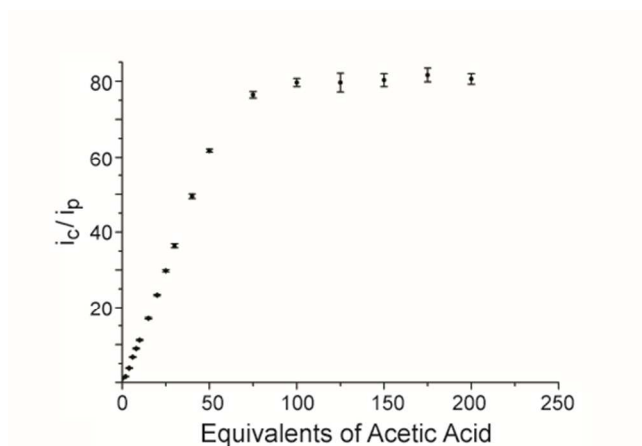
Figure 4. Dependence of normalized catalytic current, i_c , on concentration of \text{CH}_3\text{COOH} . Currents were extracted from voltammograms such as those shown in Figure 3 that were collected under the following experimental conditions: 2.0 mM 1 in THF, 0.3 M \text{TBAPF}_6 and an electrochemical potential scan rate of 100 \text{ mV s}^{-1} . Error bars indicate the standard deviation calculated from three independent measurements.
