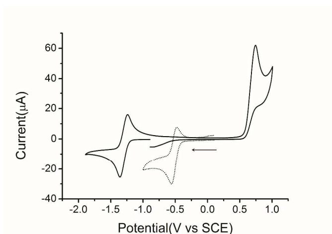
Figure 2: Cyclic voltammograms of 1 (solid line, 3 mM in THF) and 2 (dotted line, 2.7 mM) in THF at a potential scan rate of 100 \text{ mV s}^{-1} . The supporting electrolyte is 0.3 M TBAPF 6 . The arrow indicates the starting point and direction of potential cycling.
