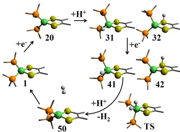
Figure 6. Proposed mechanistic scheme (based on optimized structures) for H 2 production by 1 . Green balls represent a nickel ion, orange represent phosphorous and yellow represents sulfur.
