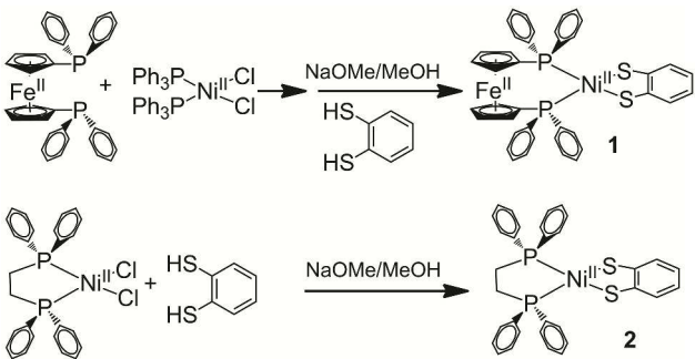
Scheme 1: Summary of synthetic procedures.
