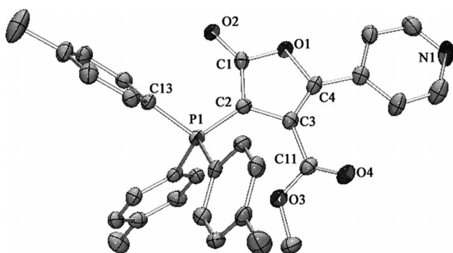
Figure 1. X-ray crystal structure of compound 3o .
