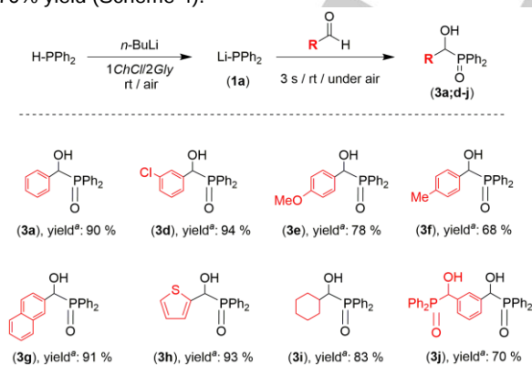
Scheme 4. Chemoselective and fast (3 s) addition of in DES prepared \text{LiPPh}_2 to various aldehydes. General reaction conditions: 1.6 mL of DES per 1.62 mmol of \text{HPR}_2 , 1.62 mmol n\text{-BuLi} and 1.62 mmol of the desired aldehyde, under air and at room temperature. The yields reported are for isolated products.
