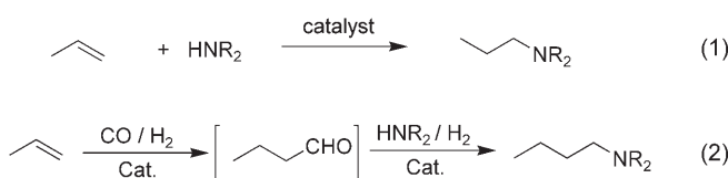
Scheme 1. Hydroamination (1) and hydroaminomethylation (2) of olefins.
