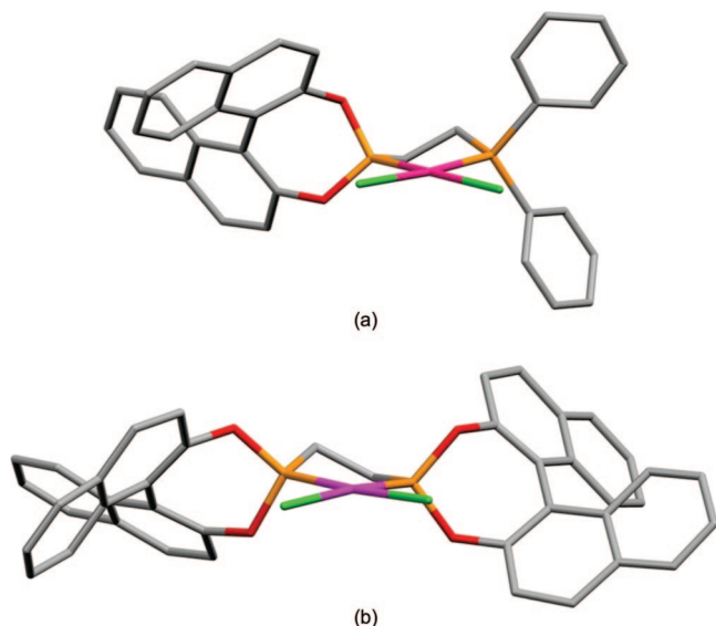
Figure 3. Crystal structures of (a) [\text{PdCl}_2(\text{L}_A)] ( 1a ) and (b) [\text{PtCl}_2(\text{L}_{2b})]^{1-} (with phenanthrene fragments truncated for ease of comparison) showing the \delta and \lambda chelate conformations and their effect on the upper-left quadrant blocking.
