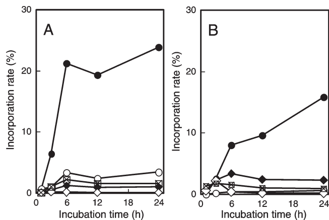
Figure 3. Feeding of ^{14}\text{C} -methionine to 6-month-old pods: (A) ^{14}\text{C} -Met (control); (B) ^{14}\text{C} -Met + unlabeled ferulic acid; \circ , vanillin; \bullet , glucovanillin; \diamond , ferulic acid; \blacklozenge , feruloyl glucosides ( cis and trans ); white box with cross, unknown 2. Decreases in fed ^{14}\text{C} -Met were not determined.
