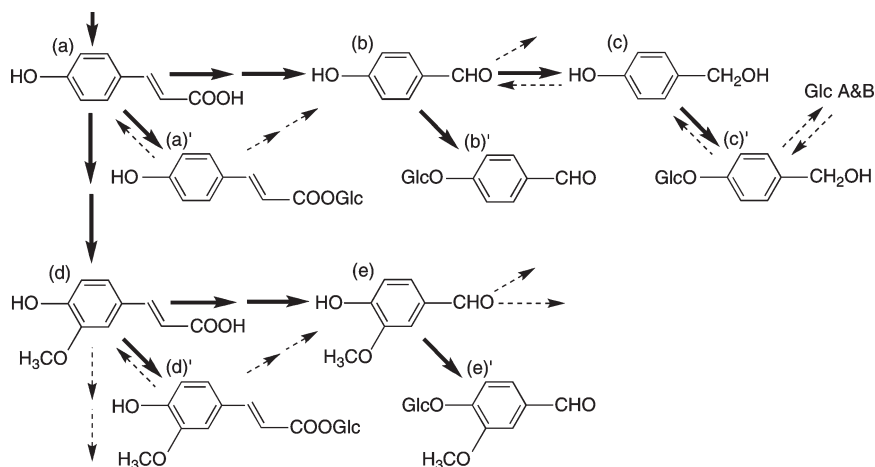
Figure 5. Proposed biosynthetic pathway for vanillin and related compounds from phenylpropanoids and formation of their glucosides and glucose esters in Vanilla planifolia : (a) 4-coumaric acid; (b) 4-hydroxybenzaldehyde; (c) 4-hydroxybenzyl alcohol; (d) ferulic acid; (e) vanillin; (a)', (b)', (c)', (d)', and (e)' show the respective glucose esters or glucosides. Glc A and B are esters of tartaric acid derivatives and two molecules of (c)' (bis[( \beta -D-glucopyranosyloxy)benzyl]-2-isopropyltartrate and bis[( \beta -D-glucopyranosyloxy)benzyl]-2-(2-butyl)tartrate, respectively). Bold and dotted arrows indicate identified and unidentified routes, respectively, in this study.
