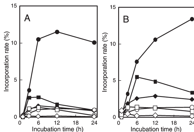
Figure 4. Feeding of ^{14}\text{C} -phenylalanine to 6-month-old pods: (A) ^{14}\text{C} -Phe (control); (B) ^{14}\text{C} -Phe + unlabeled ferulic acid; \circ , vanillin; \bullet , glucovanillin; \square , 4-coumaric acid; \blacksquare , 4-coumaroyl glucosides ( cis and trans ); \diamond , ferulic acid; \blacklozenge , feruloyl glucosides ( cis and trans ). Decreases in fed ^{14}\text{C} -Phe were not determined.
