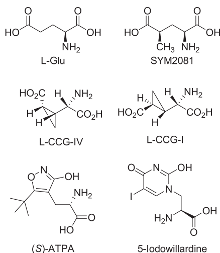
Fig. 1. Structure of model compounds.
