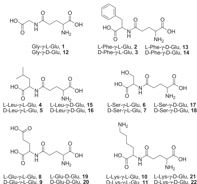
Fig. 2. Structure of target compounds.
