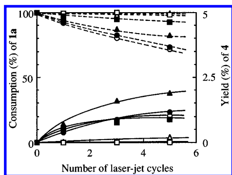
Figure 7. The dependence of the wavelength on the consumption of 1a (dashed line) and yield of 4 (solid lines). Laser power 3.5 W (total output); NB : 0.1 M. Irradiations at (i) 333 nm (○), (ii) 333 nm + 0.1 M BP (●); (iii) 351 nm (△), (iv) 351 nm + 0.1M BP (▲), (v) 364 nm (□), (vi) 364 nm + 0.1M BP (■). The results are the average of two independent runs; the experimental errors are given as Supporting Information.
