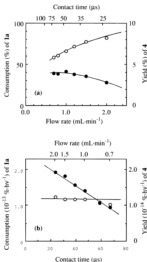
Figure 8. The dependence of the flow rate on (a) the consumption of 1a and yield of 4 and (b) the consumption of 1a and yield of 4 per photon: 1a (○), 4 (●) for one laser-jet cycle. Concentrations in acetonitrile: 1a 10^{-4} M, BP 10^{-4} M, NB 0.1 M.
