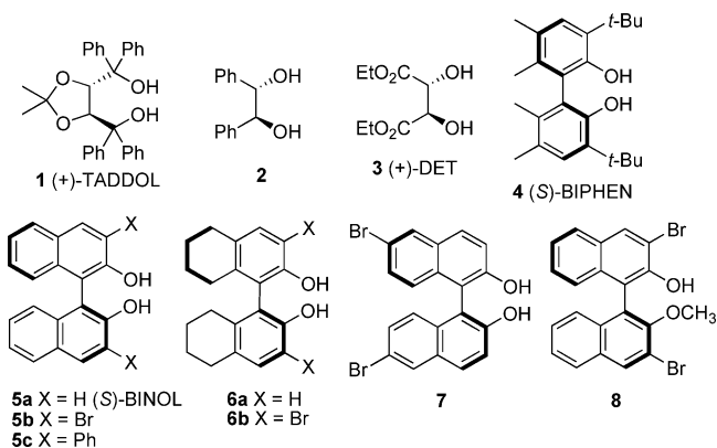
Figure 1. Chiral diols.
