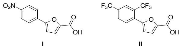
Figure 2. Chemical structures of compounds I and II.
