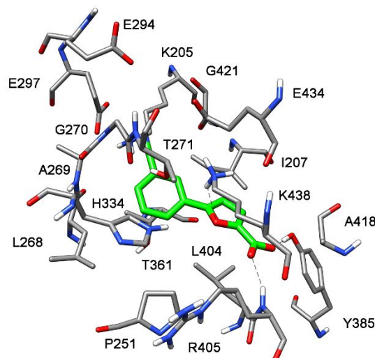
Figure 4. Minimized average structure of 10 within MbtI binding site (PDB ID 3VEH) in absence of the \text{Mg}^{2+} ion.
