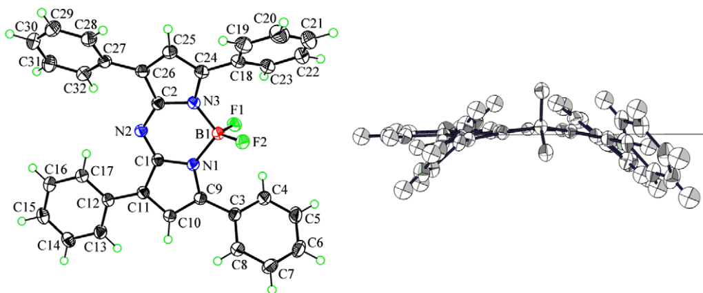
Figure 2. ORTEP view and side view of the BF 2 complex of 2a and selected bond distances (Å) and angles (°): B1–N1: 1.561(2), B1–N3: 1.553(2), N2–C1: 1.320(2), N2–C2: 1.328(2), N1–B1–N3: 105.3(1), C1–N2–C2: 119.7(1).
