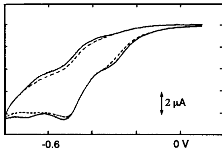
Fig. 8. Cyclic voltammograms of 3 ( c = 4.76 mM) in MeOH (0.1M LiCl, 0.06M HCl) at 20° in the absence (---) and presence (—) of acenaphthylene ( c = 43 mM). Scan rate 0.1 V s -1 .
