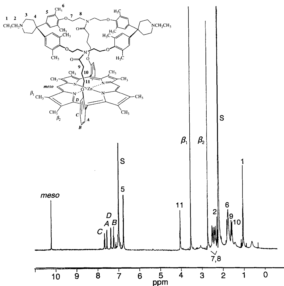
Fig. 1. 500-MHz ^1\text{H} -NMR Spectrum of 2 in p -( \text{D}_{10} )xylene. T 383 K; S = solvent; arbitrary numbering.
