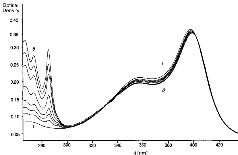
Fig. 7. UV/VIS Titration of 3 ( c = 2.0 \cdot 10^{-5} \text{ mol l}^{-1} ) with phenanthrene (spectrum 1: c = 1.4 \cdot 10^{-5} \text{ mol l}^{-1} ; spectrum 8: 1.0 \cdot 10^{-4} \text{ mol l}^{-1} ) in \text{CF}_3\text{CH}_2\text{OH} at 293 K. d = 1 \text{ cm} .
