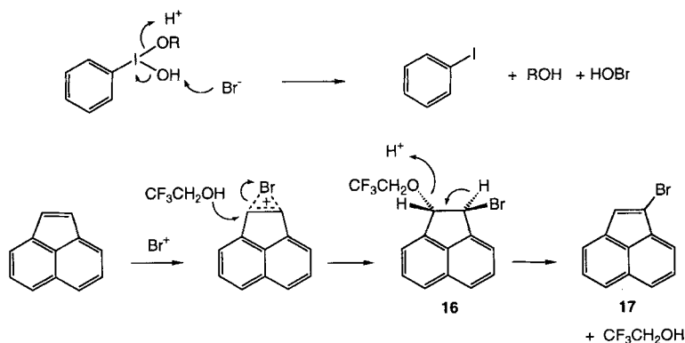
Scheme 4. Possible Mechanism for Formation of \text{HOBr} and Reaction with Acenaphthylene in \text{CF}_3\text{CH}_2\text{OH}
