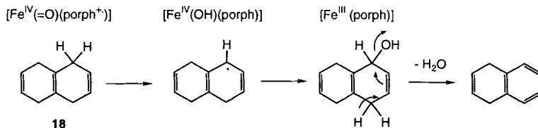
Scheme 5. Possible Mechanism for the Aromatization of Isotetralin ( 18 ) in the Reaction with \text{PhIO} and 3 ( 3 \text{ SbF}_6^- instead of 3 \text{ Br}^- ) in \text{CF}_3\text{CH}_2\text{OH}
