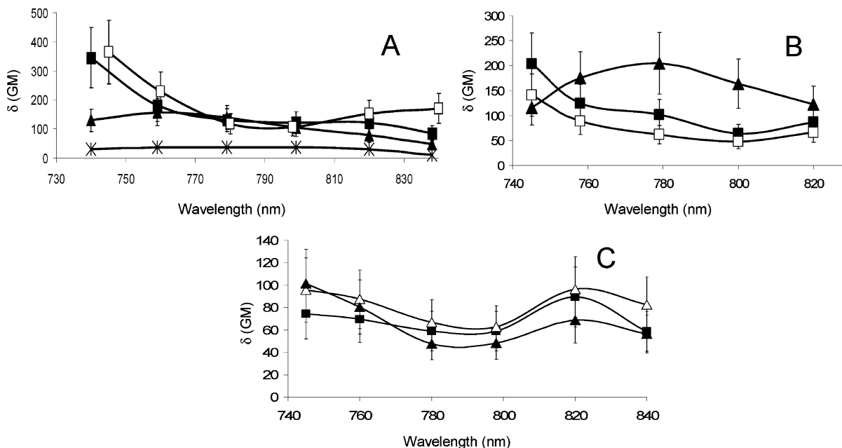
FIGURE 3. Two-photon absorption cross sections of compounds in dichloromethane and fluorescein (*) in aqueous KOH (pH 10–11): (A) benzothiazole series 28c (TP-2Bz, ▲), 29c (TP-3Bz, ■), 37 (TP-3Bz O-alkyl-ester, □); (B) biscyano series 28a (TP-2BCN, ▲), 29a (TP-3BCN, ■), 21 (TP-3BCN-OMe, □); and (C) pyridine series 28b (TP-2Py, ▲), 29b (TP-3Py, ■), 22 (TP-3Py -COOMe, △).
