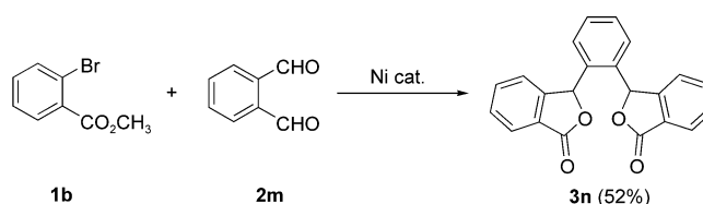
Scheme 3. Synthesis of a diphtalide derivative.
