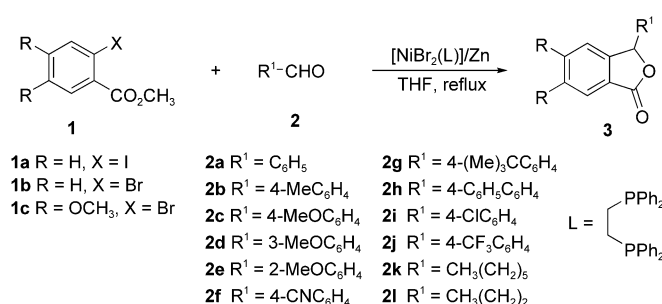
Scheme 2. Nickel-catalyzed cyclization reaction to produce phthalides.
