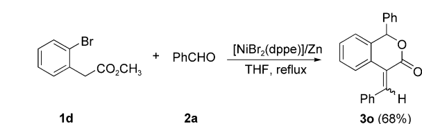
Scheme 4. Synthesis of a six-membered lactone.
