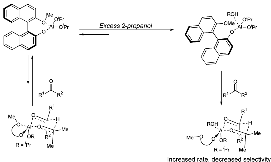
SCHEME 6. Proposed Scheme Showing the Dissociation of the Al–Ether Dative Bond in the Complex Formed between (S)-5 and AlMe 3 in the Presence of Excess 2-Propanol
