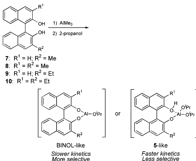
SCHEME 7. Possible Modes of Reactivity between AlMe 3 and the Substituted BINOL Derivative (S)-7 through (S)-10
