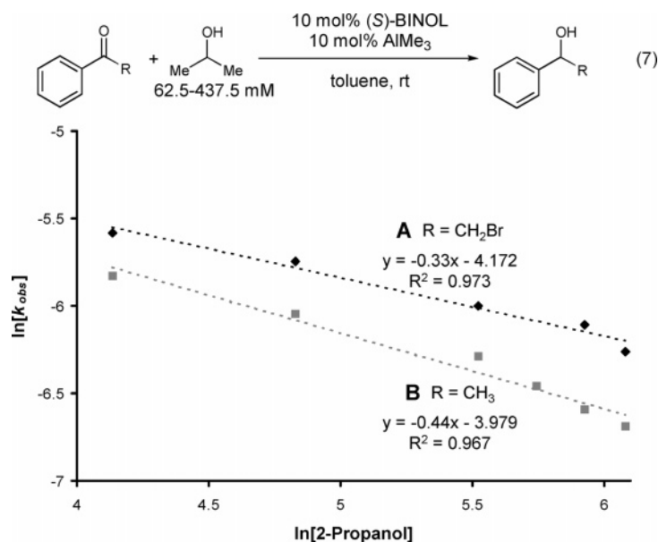
FIGURE 7. Plot of \ln[k_{\text{obs}}] versus \ln[2\text{-propanol}] for the (BINOL)Al-catalyzed MSPV reduction of \alpha -bromoacetophenone (R = CH 2 Br, A) and acetophenone (R = CH 3 , B) with 2-propanol.
