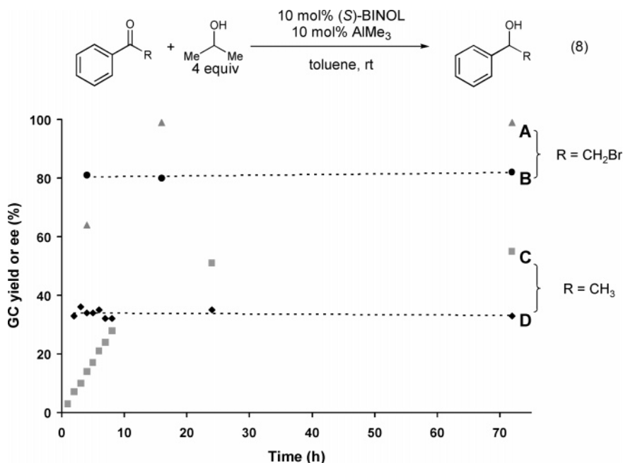
FIGURE 8. Reaction yield ( \blacktriangle and \blacksquare , grey) and product ee ( \bullet and \blacklozenge ) as a function of time for the MSPV reduction of \alpha -bromoacetophenone (R = CH 2 Br; yield line A ( \blacktriangle ); ee line B ( \bullet )) and acetophenone (R = CH 3 ; yield line C ( \blacksquare ); ee line D ( \blacklozenge )) catalyzed by (S)-BINOL/AlMe 3 .
