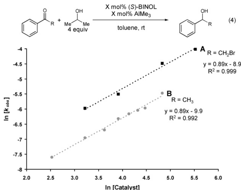
FIGURE 4. Plots of \ln[k_{\text{obs}}] versus \ln[\text{catalyst}] for the (BINOL)Al-catalyzed MSPV reduction of \alpha -bromoacetophenone ( \text{R} = \text{CH}_2\text{Br} , A) and acetophenone ( \text{R} = \text{CH}_3 , B) with 2-propanol.
