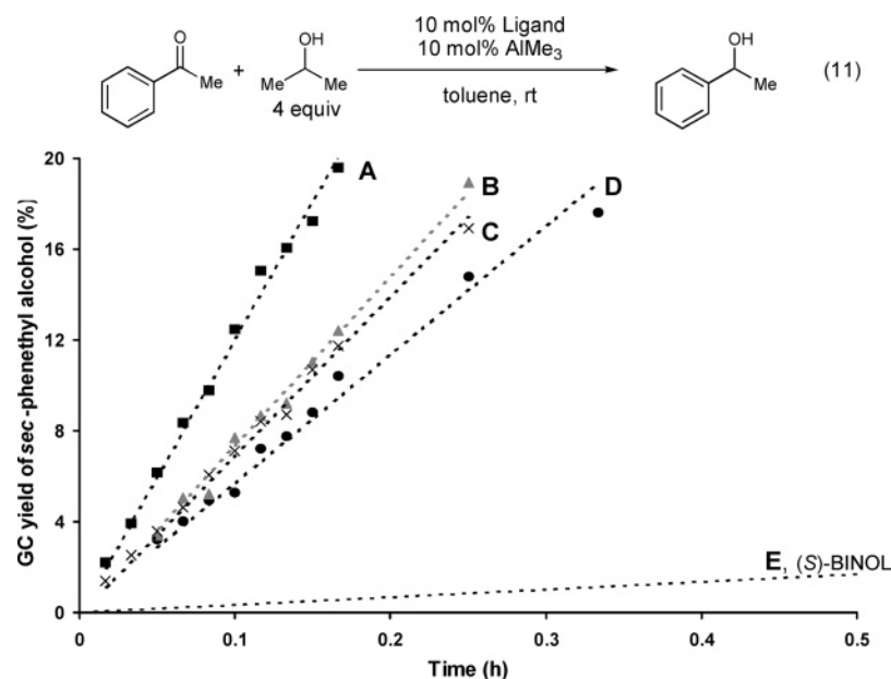
FIGURE 11. Initial reaction rates of the MSPV reduction of acetophenone with 2-propanol, using (S)-7/AlMe 3 (D), (S)-8/AlMe 3 (A), (S)-9/AlMe 3 (B), (S)-10/AlMe 3 (C), and (S)-BINOL (E) as the catalytic precursors. Line E was generated from the rate data obtained for (S)-BINOL in Figure 3.
