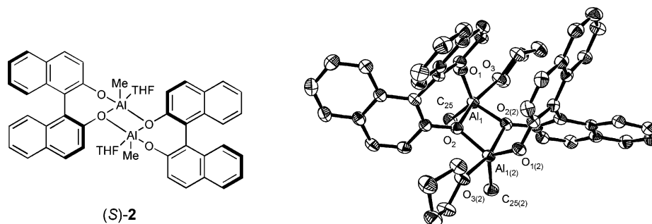
FIGURE 1. An ORTEP depiction of the crystal structure of the isolated aluminum dimer (S)-2 showing the atom labeling scheme and the asymmetric subunit. Thermal ellipsoids are drawn at 50% probability. Hydrogens are omitted for clarity.
