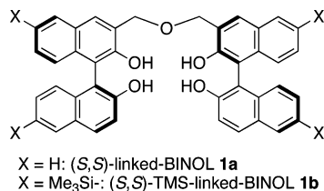
Figure 1. Structures of (S,S)-linked-BINOL 1a and (S,S)-TMS-linked-BINOL 1b .
