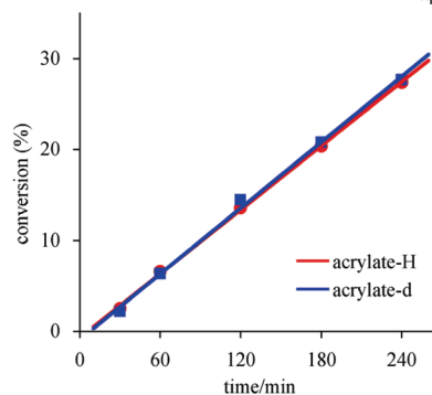
Figure 2. Kinetic isotope effect study using deuterated methyl acrylate d -3.
