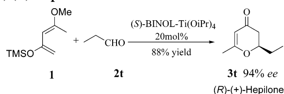
SCHEME 1. One-Step Synthesis of ( R )-(+)-Hepialone
