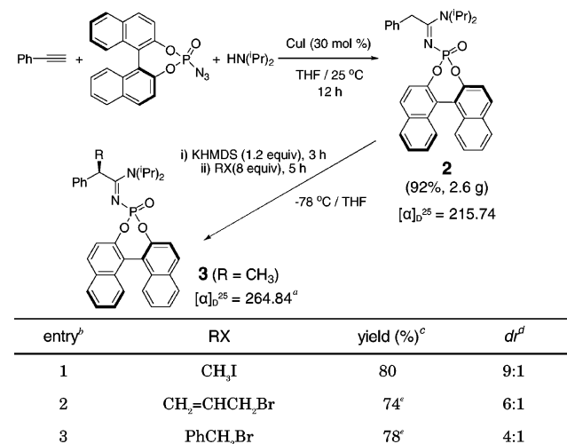
SCHEME 1. Amidine Synthesis with Chiral Binaphthol Azide and Subsequent Alkylation at the \alpha -Position of the Amidine
