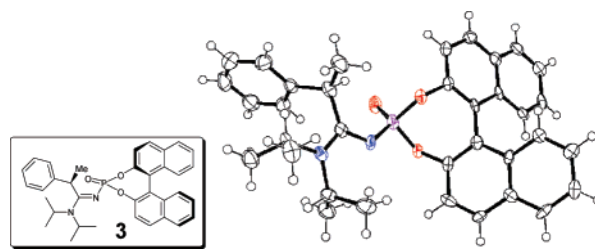
FIGURE 1. ORTEP of an \alpha -methylated amidine 3 .
