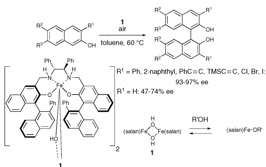
Scheme 1. Iron(salan)-Catalyzed Asymmetric Aerobic Oxidative Coupling of 2-Naphthols
