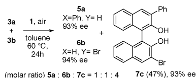
Scheme 4. Cross-Coupling of Two 3-Substituted 2-Naphthols
