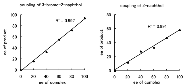
Figure 2. Relationship between the enantiomeric excesses of catalyst 1 and the coupling product.
