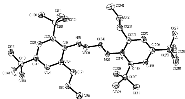
Figure 2. ORTEP diagram of LH 4 . Thermal ellipsoids are shown at 50% probability. Hydrogen atoms are omitted for clarity.
