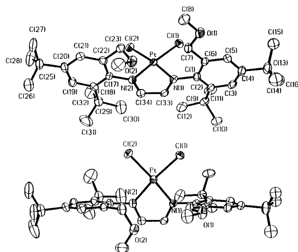
Figure 3. ORTEP diagrams of \text{LPtCl}_2 ( 2b ). Thermal ellipsoids are shown at 50% probability. Hydrogen atoms are omitted for clarity.
