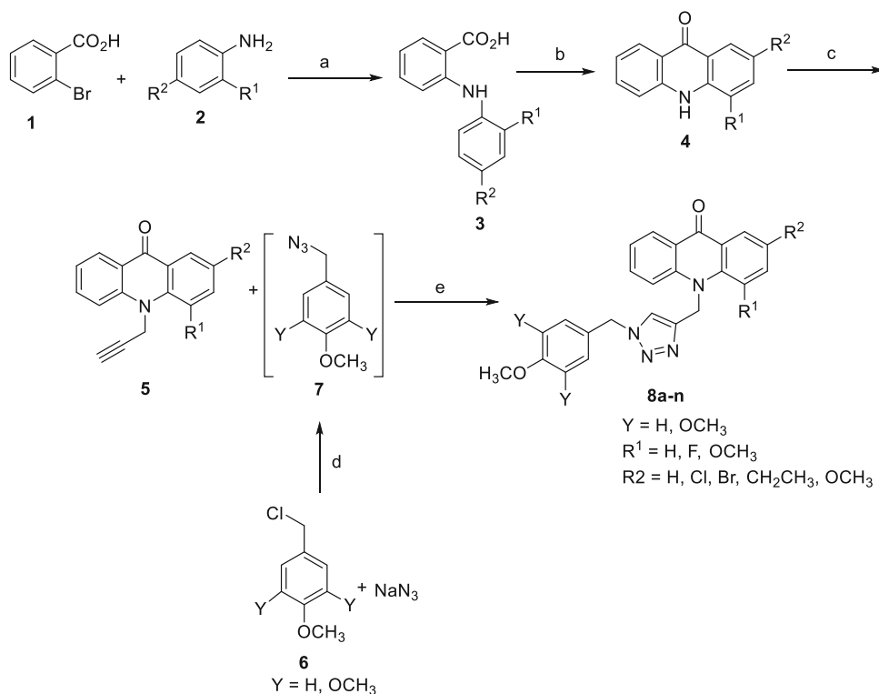
Scheme 1 Synthesis of compounds 8a–n . Reagents and conditions: a K_2CO_3 , Cu, EtOH, reflux, 7 h; b PPA, 100 °C, 3 h; c propargyl bromide, KOtBu , DMSO, rt, 3 h; d NEt_3 , H_2O/t -BuOH (1:1), rt; e CuI , 24–56 h
